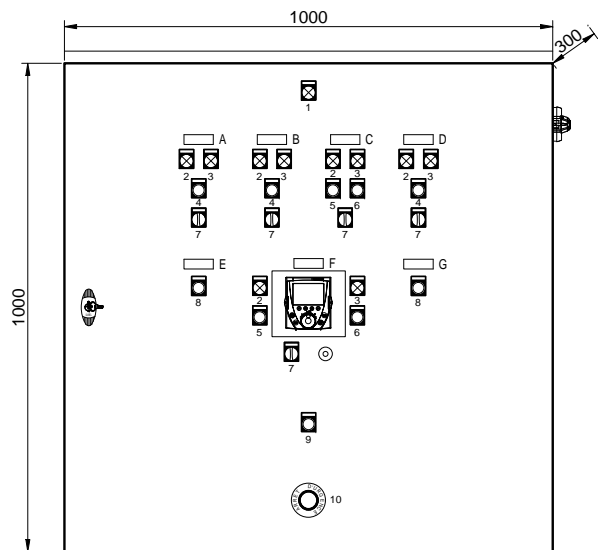
IMPLANTATION FACADE
