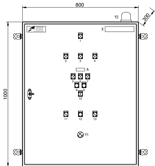
FACADE EXTERNE
