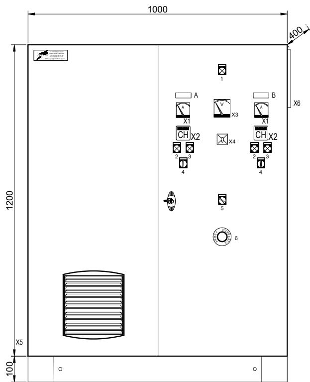
IMPLANTATION FACADE
