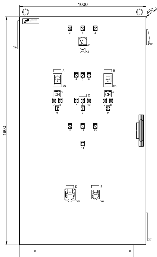
IMPLANTATION FACADE
