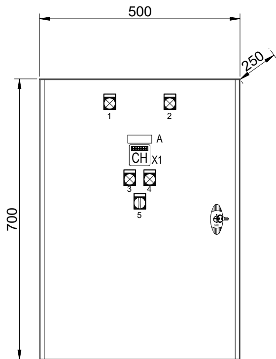
IMPLANTATION FACADE
