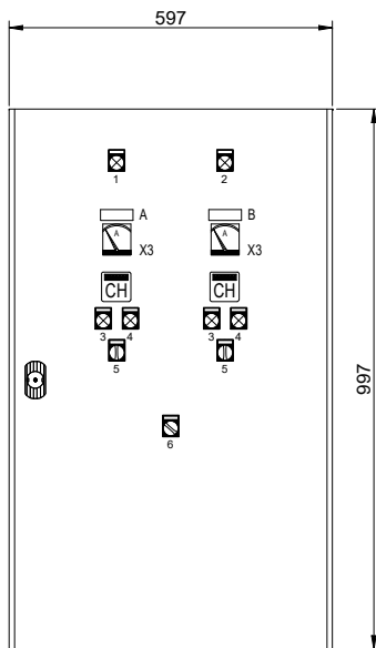
IMPLANTATION FACADE PORTE INTERIEURE
