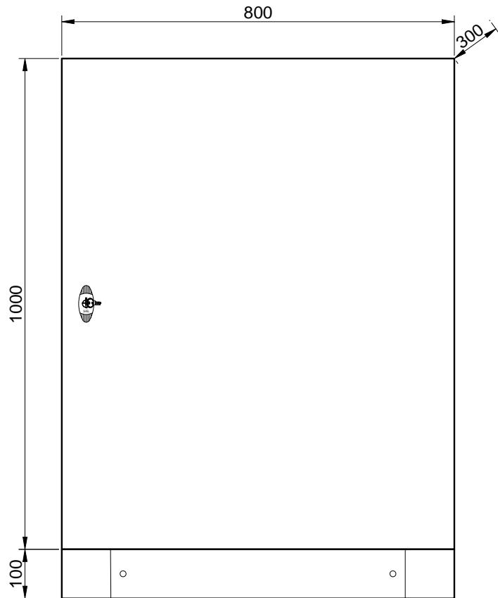
IMPLANTATION FACADE
