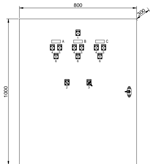
IMPLANTATION FACADE
