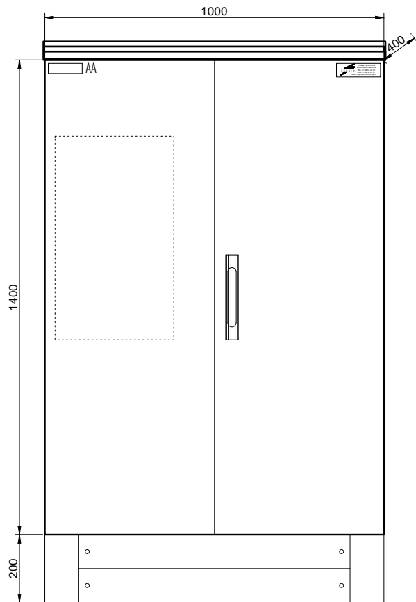
FACADE EXTERNE
