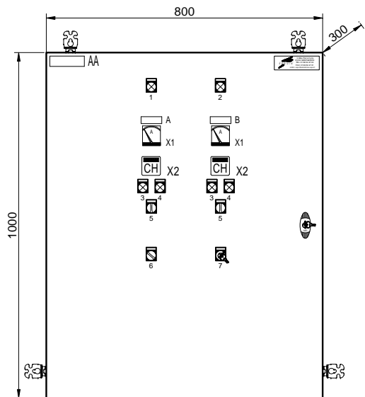
FACADE EXTERNE
