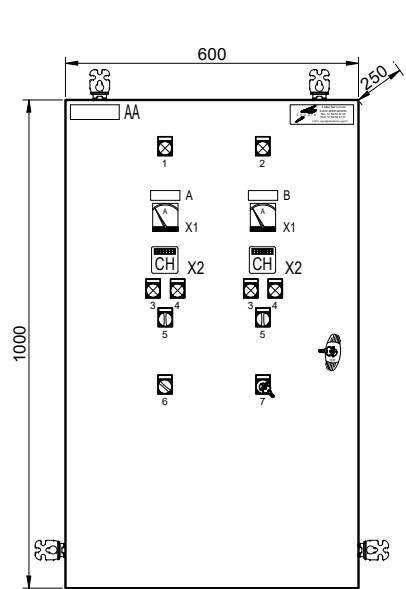
IMPLANTATION FACADE
