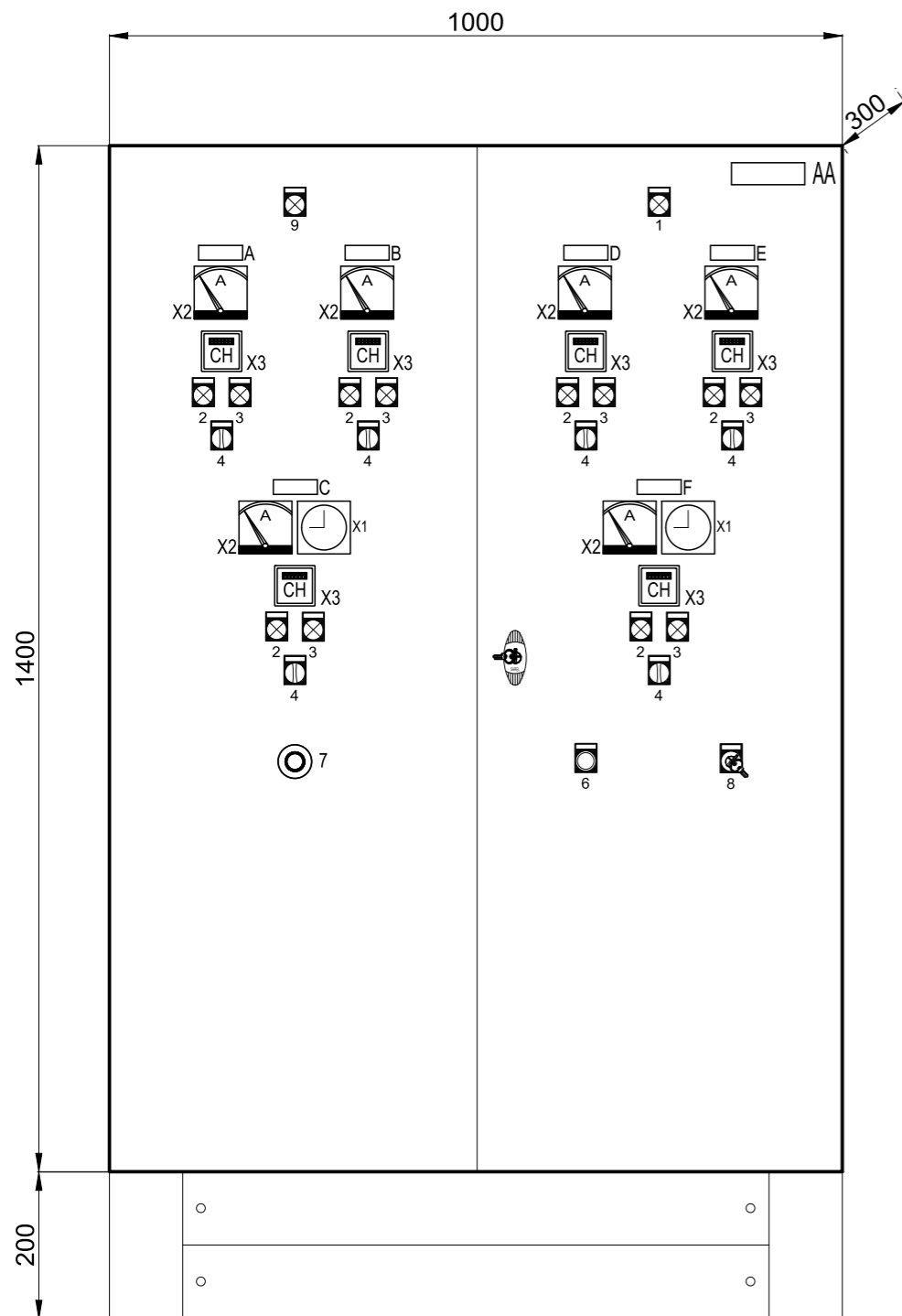
IMPLANTATION FACADE
