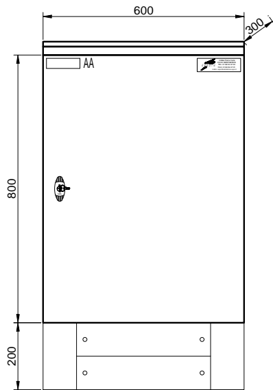
IMPLANTATION FACADE EXTERNE
