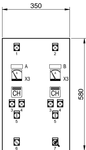
IMPLANTATION FACADE PLATINE INTERIEURE
