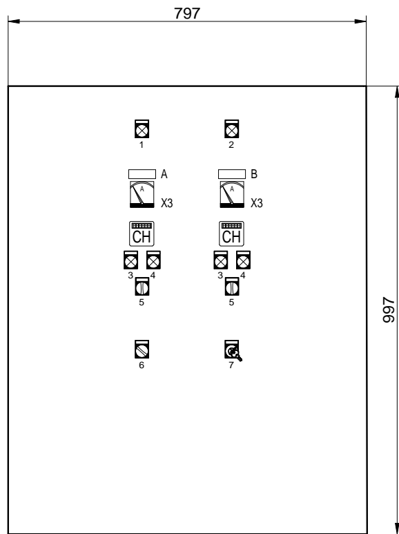
IMPLANTATION FACADE PORTE INTERIEURE
