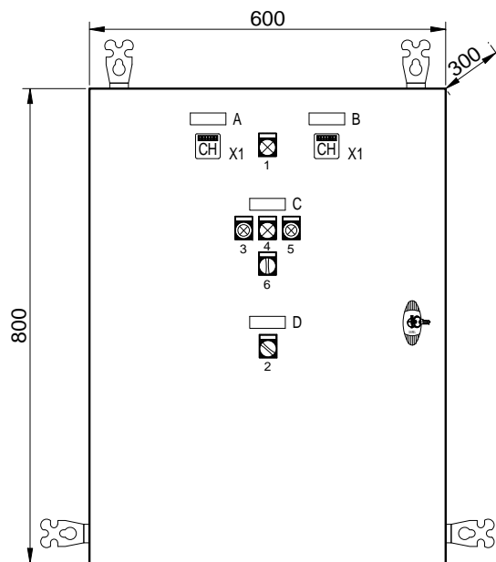
IMPLANTATION FACADE
