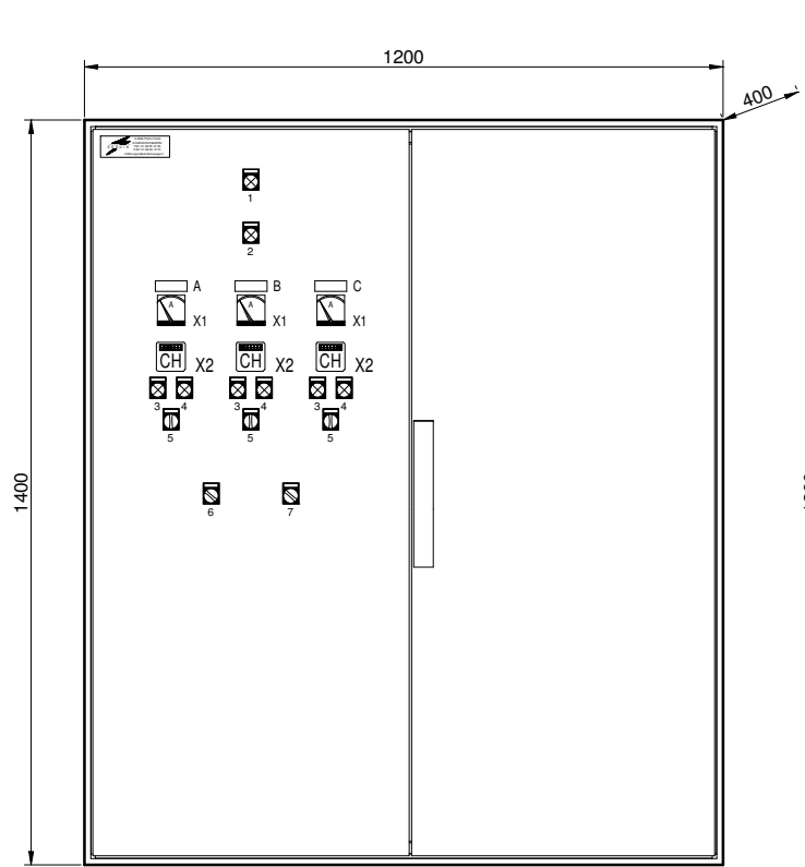
FACADE
