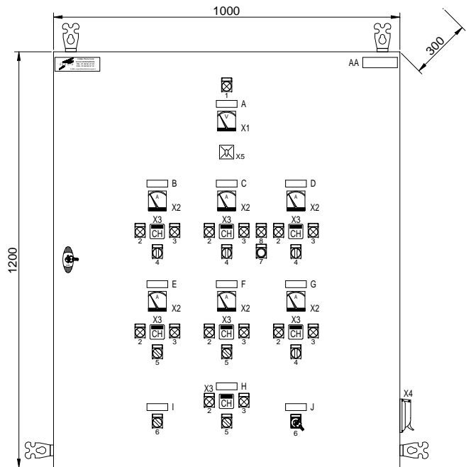
FACADE COFFRET ELECTRIQUE
