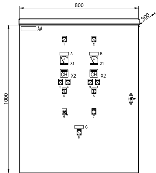
FACADE
