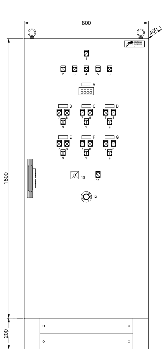
IMPLANTATION FACADE
